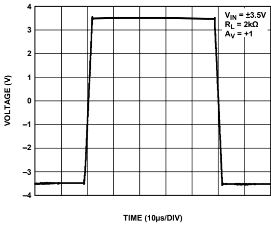
Figure 16. Large Signal Transient Response, V_{SY} = \pm 5V
