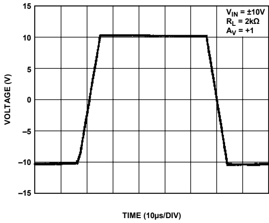
Figure 15. Large Signal Transient Response, V_{SY} = \pm 15V
